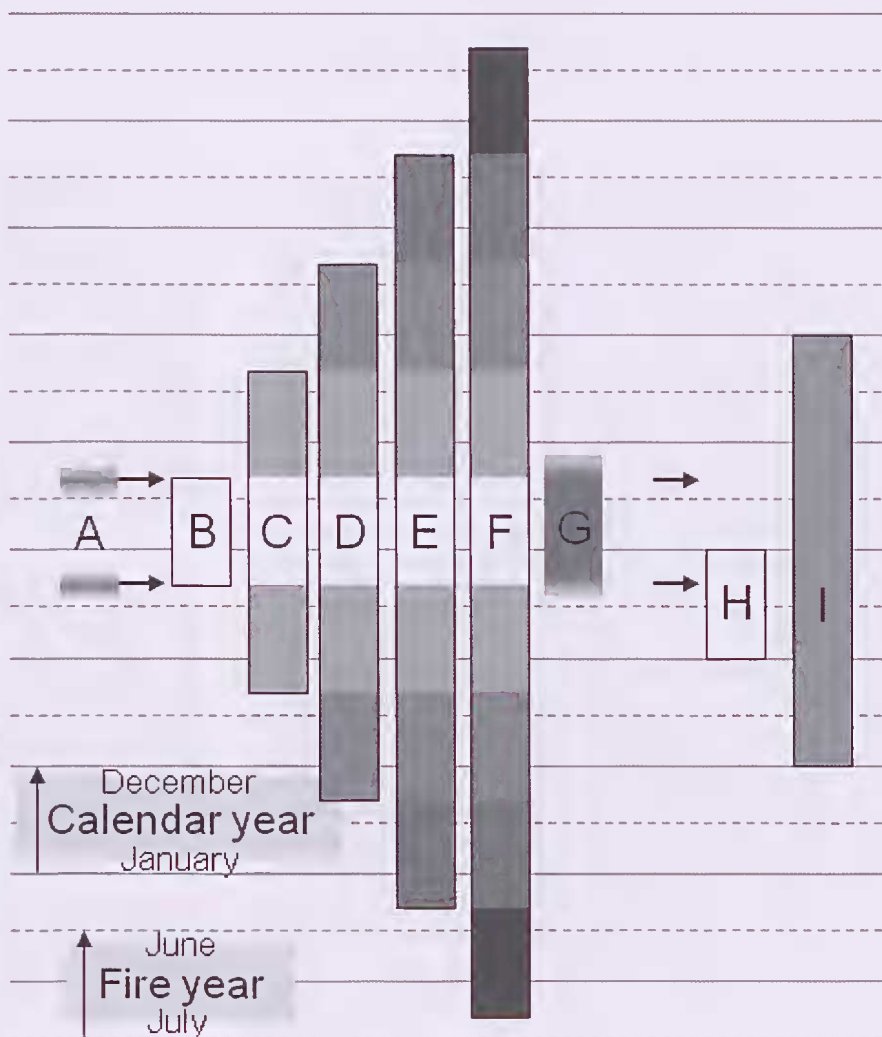
Figure 1 Comparison of census years and precision windows for grasstree and satellite records considered by Miller et al. (2007) (A–G), versus those of Ward (2009) (H–I). Satellite image dates (A) define the satellite census year (B) but vary with availability around August–September (arrows delimit one sample year). Miller et al. analysed varying degrees of temporal precision by resizing a symmetric window of agreement around each fire record to 1, 3, 5, 7 and 9 years (B–F). While the duration of grasstree annual banding is not known, in southwest Australia grasstree phenology changes from a slow to a fast growth phase in late winter/early spring (Lamont et al. 2004, Korczynskyj & Lamont 2005), suggesting a grasstree growing year (G) similar to the satellite year. Ward implicitly assumed grasstree year = calendar year (H) and takes this as the census year. As each of these overlap two satellite years, Ward (2009 p. 262) allowed ‘[grasstree fire dates] a tolerance of a calendar year either way, and fires dated from satellite images a year’s extension backwards’—an offset asymmetrical agreement window of four years (I).
